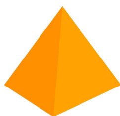
square pyramid
