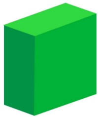
cuboid
