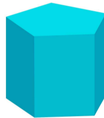
pentagonal prism
