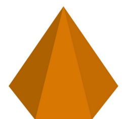
hexagonal pyramid
