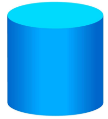
cylinder
