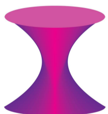
hyperboloid
